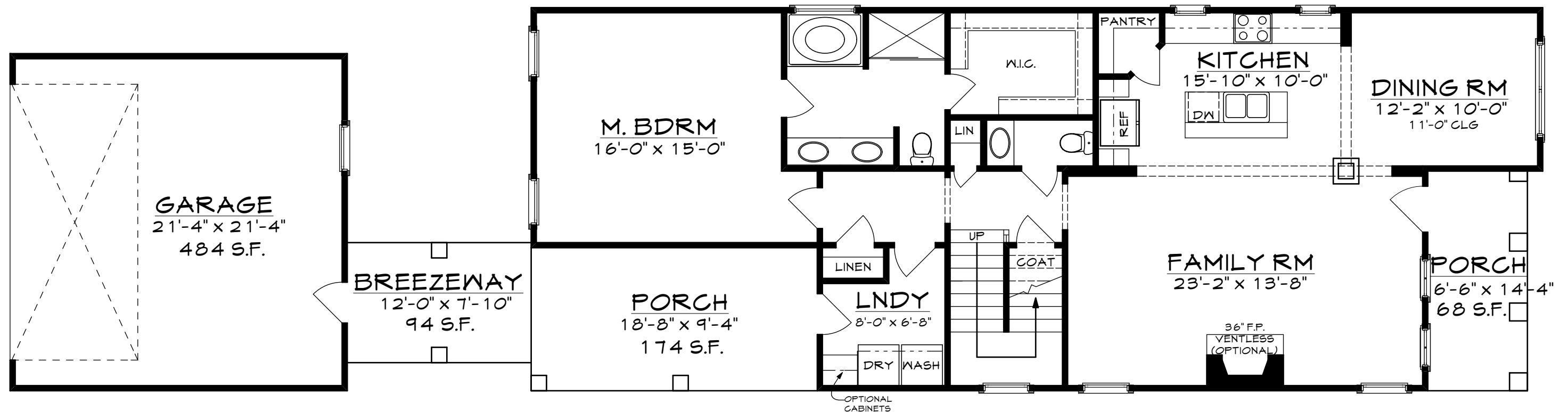
FIRST FLOOR PLAN 1396 SF HTD. 9'-0" CEILINGS
