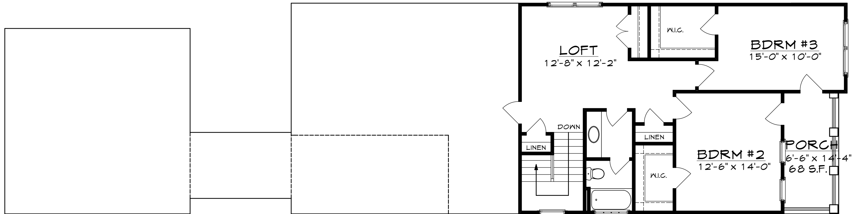
SECOND FLOOR PLAN 802 SF HTD. 8'-0" CEILINGS
