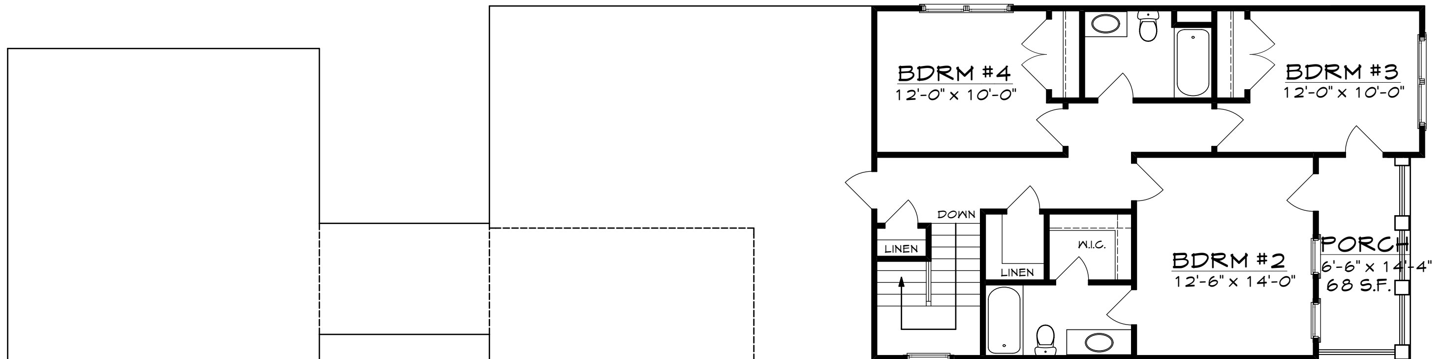
SECOND FLOOR PLAN W/ 4 TH BEDROOM OPTION
