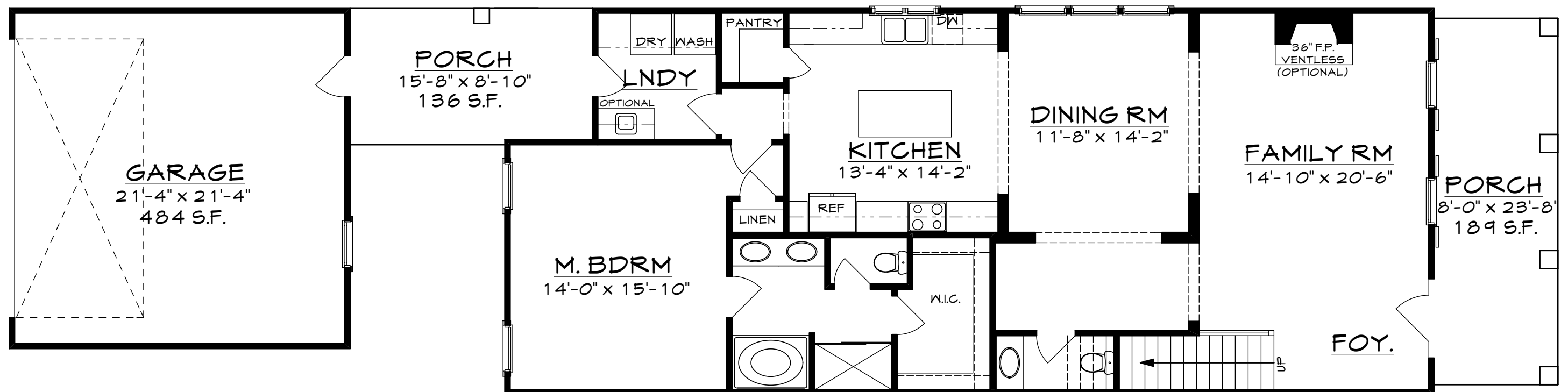
FIRST FLOOR PLAN 1452 S.F. HTD. 9'-0" CEILINGS
