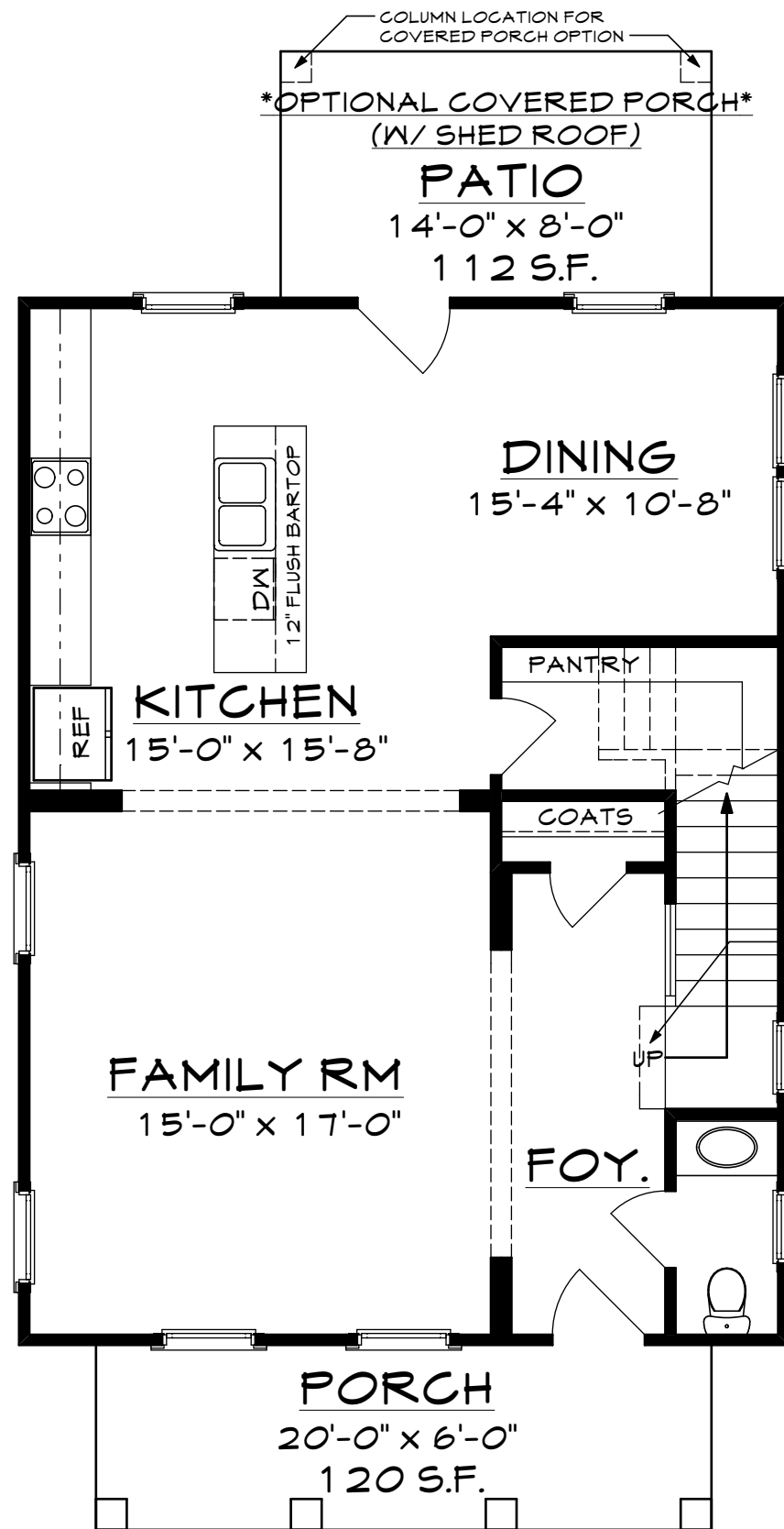
FIRST FLOOR PLAN 850 SF HTD. 9'-0" CEILINGS (OPTIONAL 10'-0")
