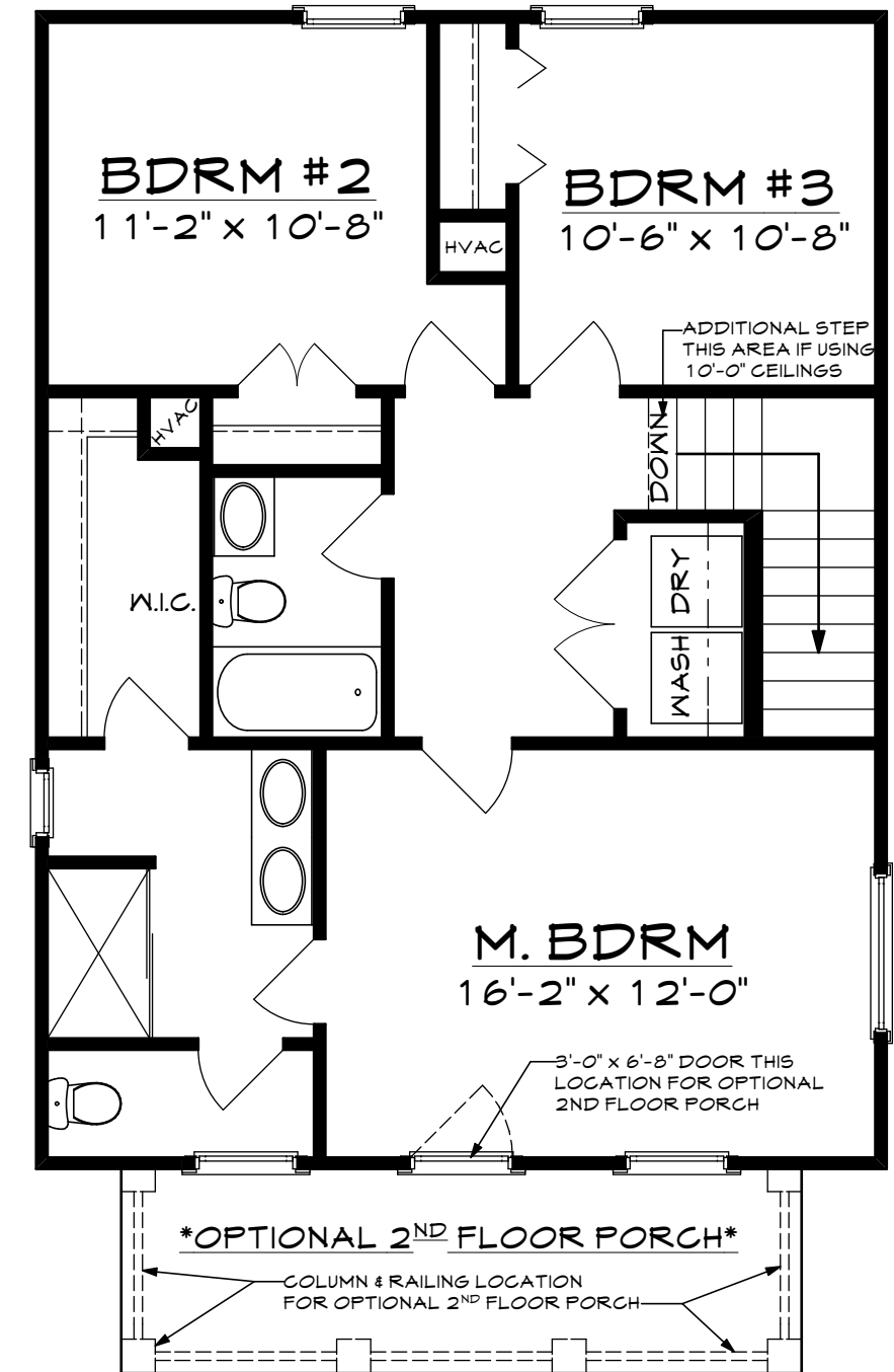
SECOND FLOOR PLAN 800 SF HTD. 8'-0" CEILINGS (OPTIONAL 9'-0")
