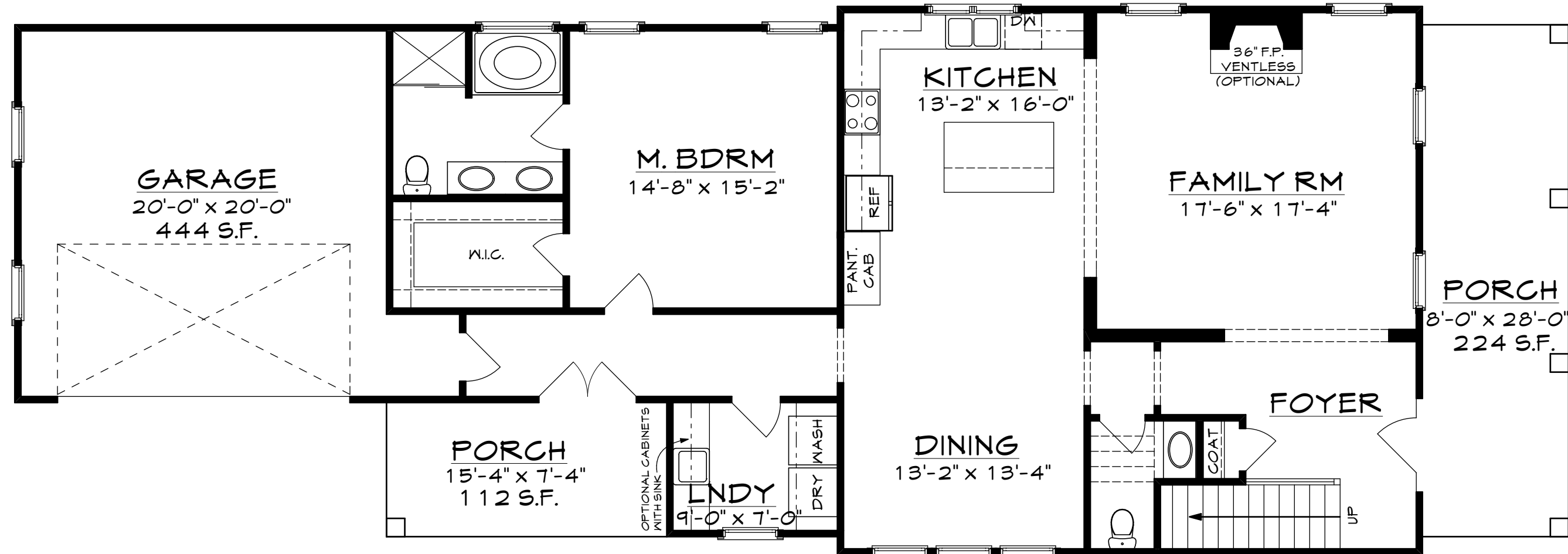
FIRST FLOOR PLAN 1515 SF HTD. 9'-0" CEILINGS
