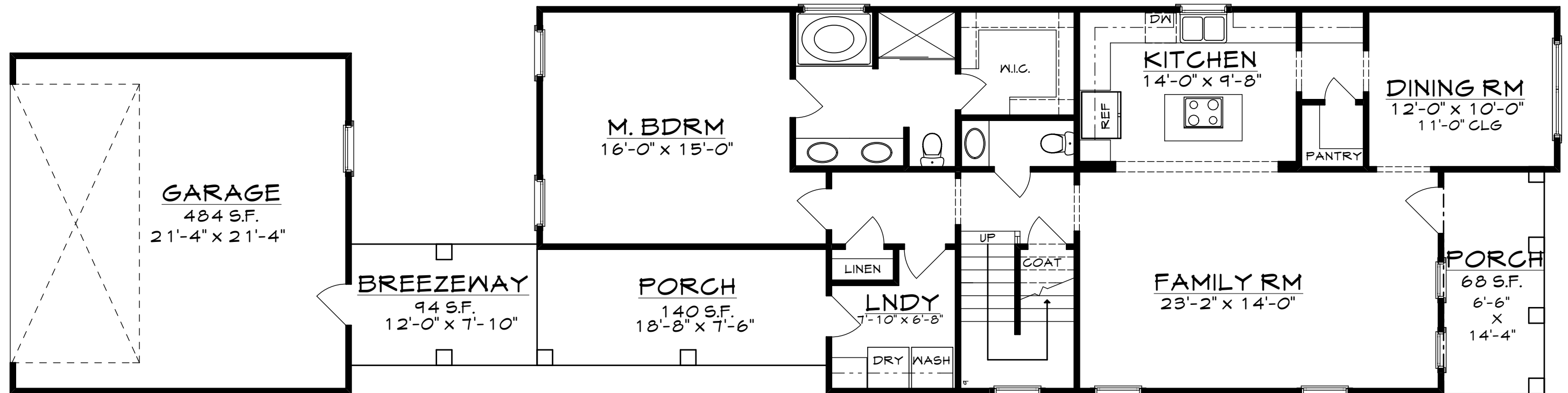
FIRST FLOOR PLAN 1396 SF HTD. 9'-0" CEILINGS
